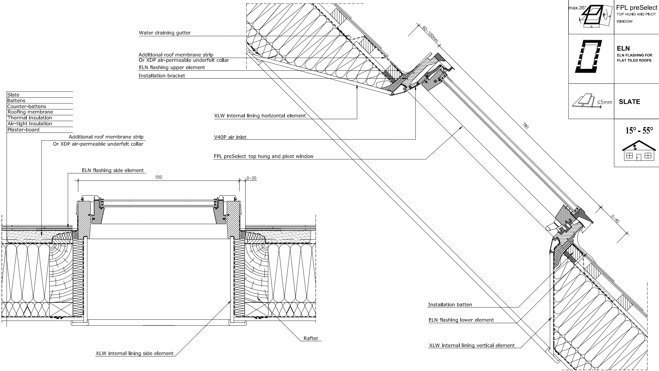
Vertical and horizontal cross-section: FPL preSelect top hung and pivot window with ELN flashing for flat tiled roofs.
